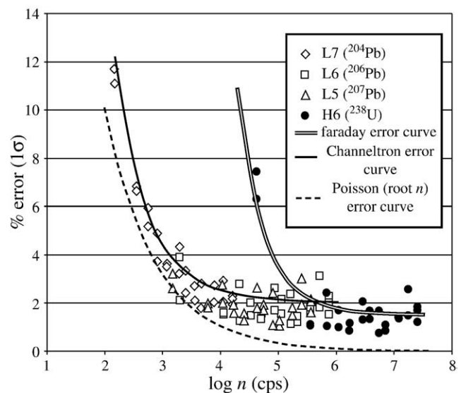
Fig. 6. Relationship between average counts per second (not blank – corrected) and 1 \sigma error from sets of 30 one-second integrations measured on Channeltron and faraday detectors throughout the linearity experiments. Also plotted are visual-fit error calibration curves used to calculate errors during laser acquisition; an additional error curve based on root n is plotted for reference.
