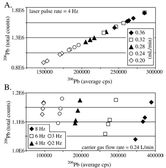
Fig. 3. The relationship between average counts per second and total integrated counts ^{206}\text{Pb} on standard Sri Lanka Zircon using 24 laser pulses with variable A) carrier gas flow and B) laser hit pulse rate.
